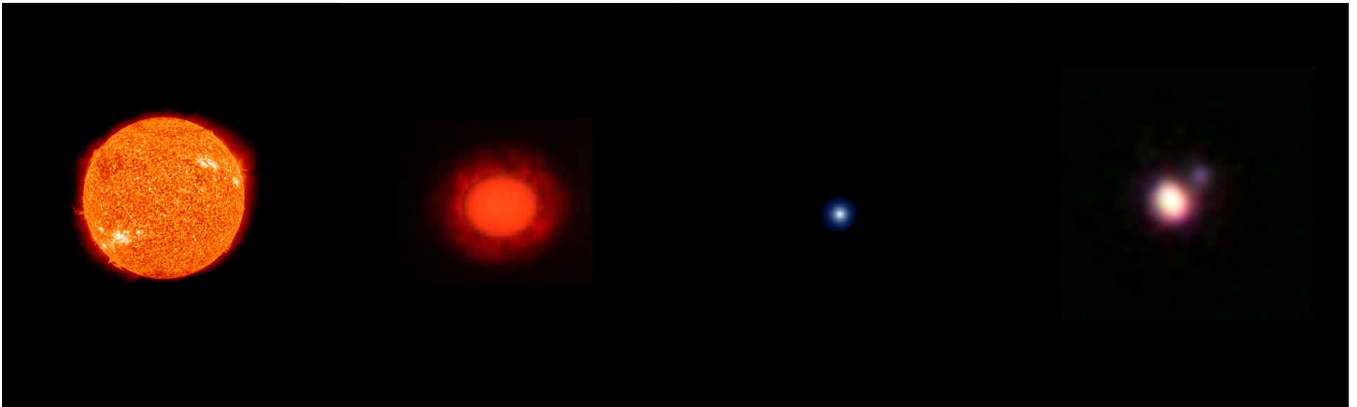
yellow dwarf
